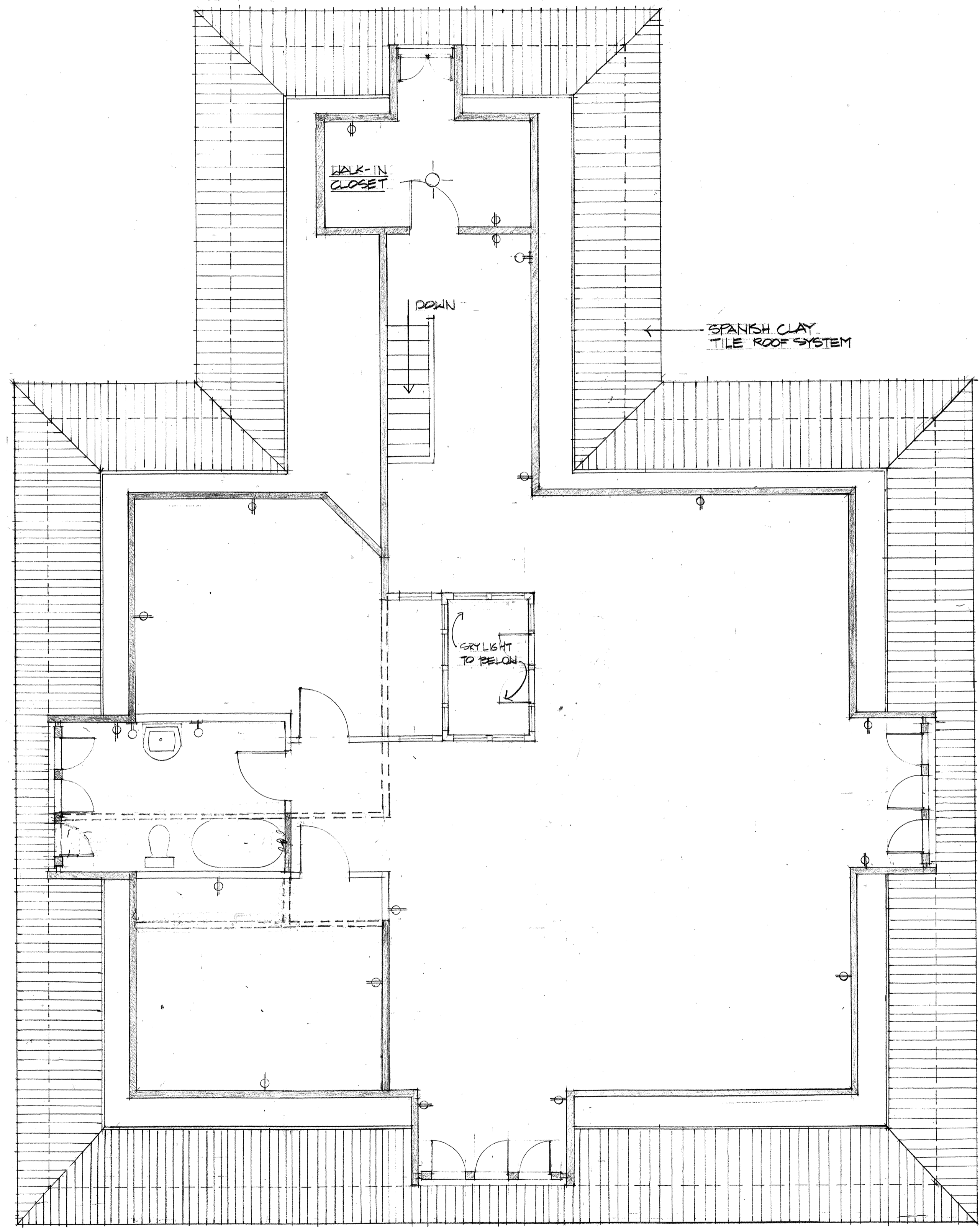
ATTIC FLOOR PLAN 1/4" = 1'-0" NORTH
